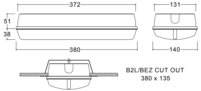
Dimensions (mm)
